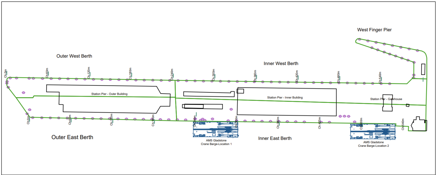
SITE PLAN
