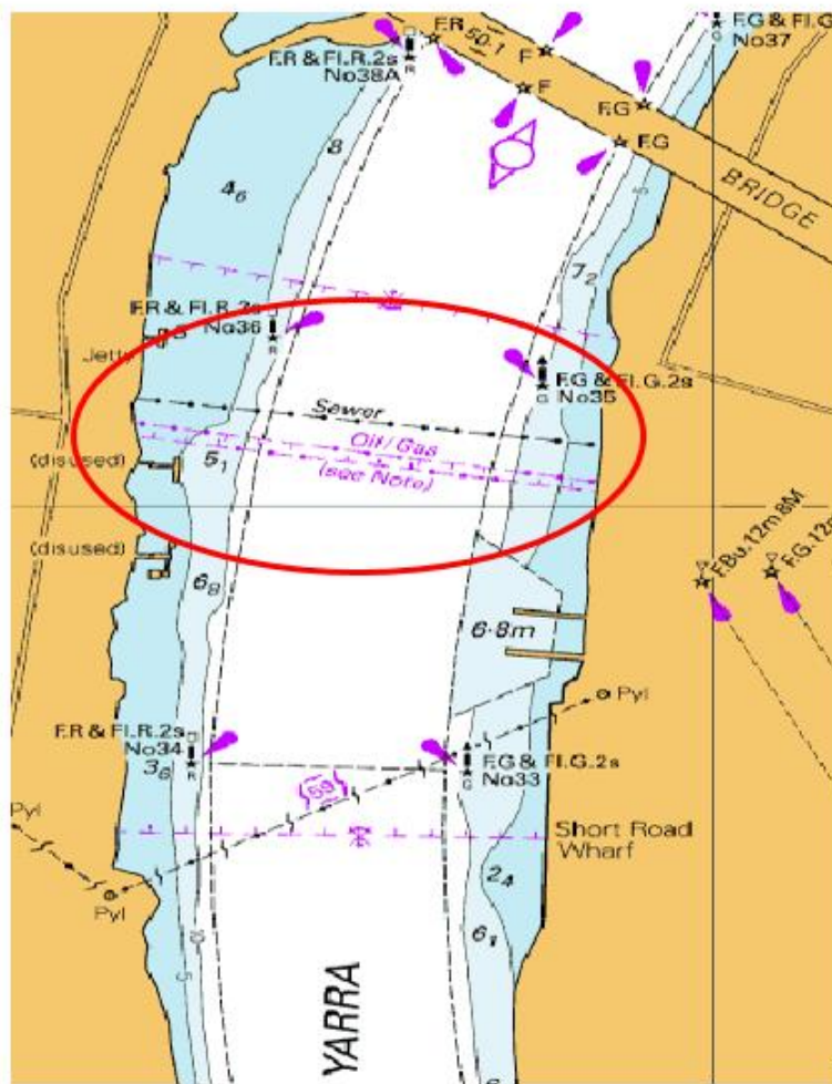
Hobsons Bay Main Sewer protection plates between Yarra River Beacons 33/34 and 35/36
